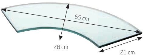
buffet platter Curve 90° hardened clear glass, 10 mm thick, curved shape, edges polished and deburred
